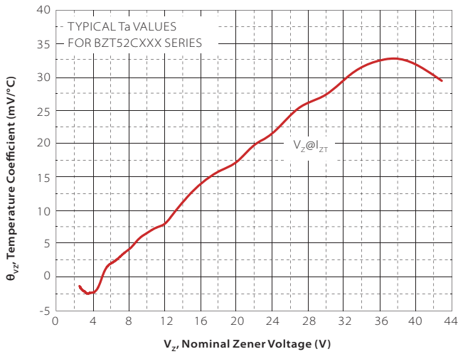
Temperature Coefficients
